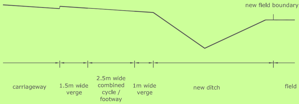
TYPICAL CROSS SECTION OF PROPOSED COMBINED CYCLE/FOOTWAY
